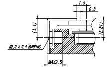
SECTION D-D' (S:5/1)
